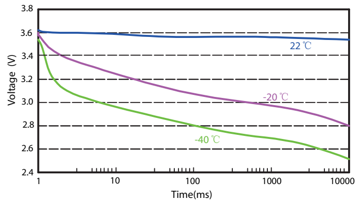
UPC1550 500mA Discharge Curve
