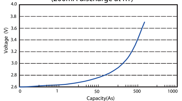
UPC1550 Capacity vs.OCV (200mA discharge at RT)
