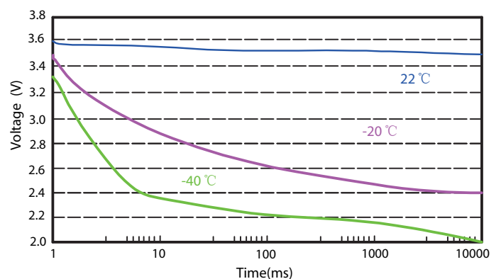
UPC1550 1000mA Discharge Curve
