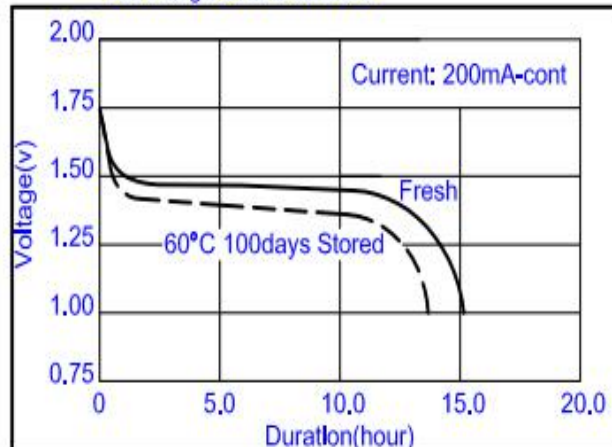
Discharge Characteristics
