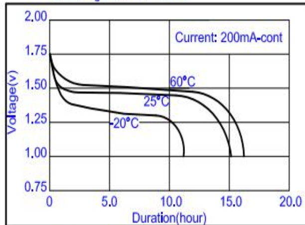
Discharge Characteristics
