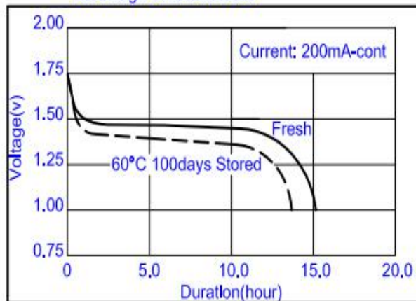
Discharge Characteristics
