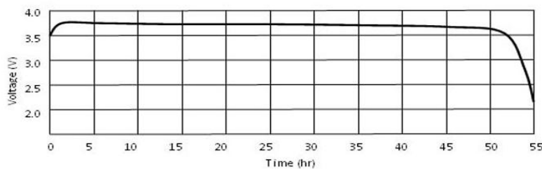
ER33615MS150 cell on 200mA at 150°C Discharge Curve
