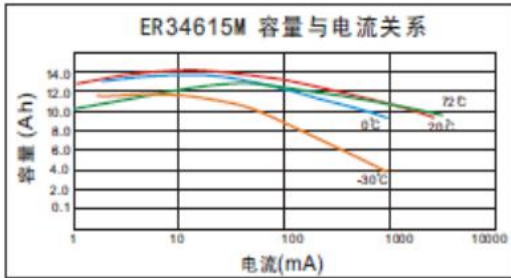
Capacity VS Current curve
