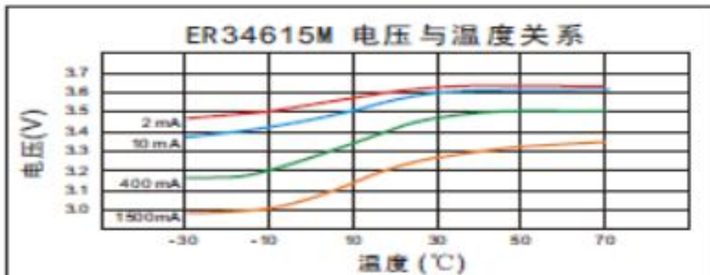
Voltage VS Temperature curve
