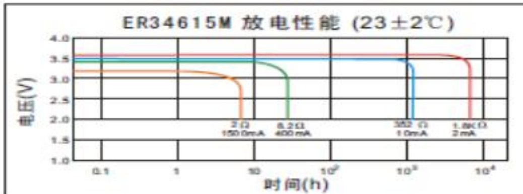
Voltage VS Time curve
